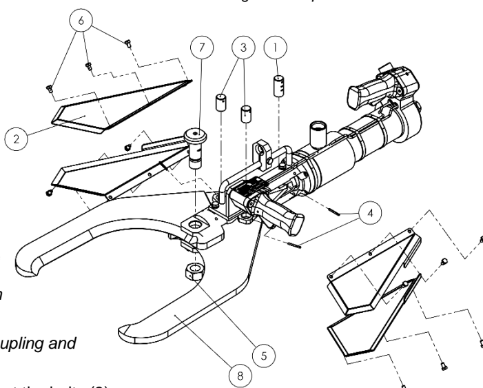
Fig. 7.1 – Exploded view
