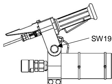
Abb. 5.8 Handle holder
