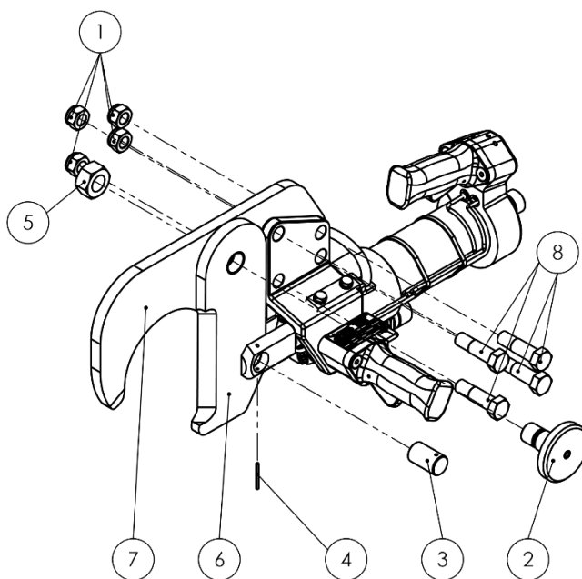
Fig. 7.1 – Exploded view
