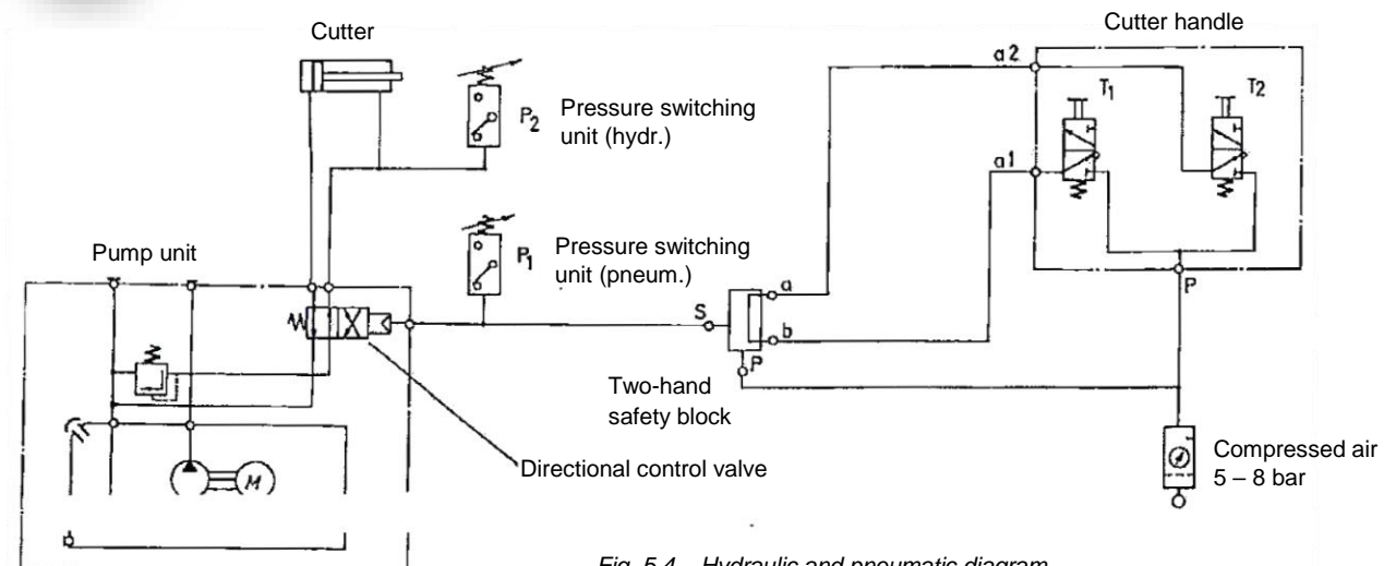
Fig. 5.4 – Hydraulic and pneumatic diagram
