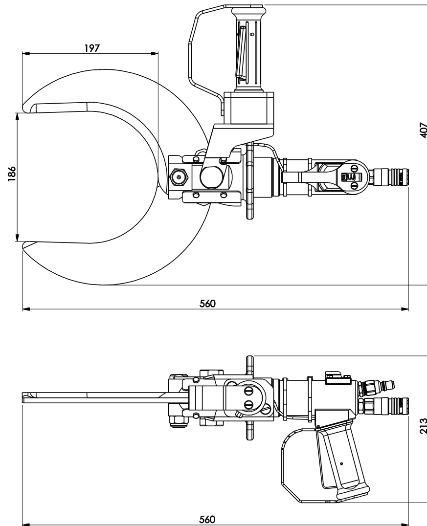
Dimensional drawing
