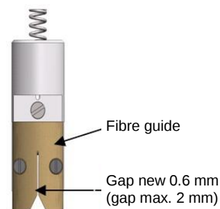
Fig. 7.3 – Changing guide
