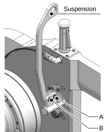
Fig. 5.3 – Suspension
