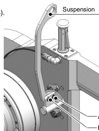
Fig. 5.3 – Suspension
