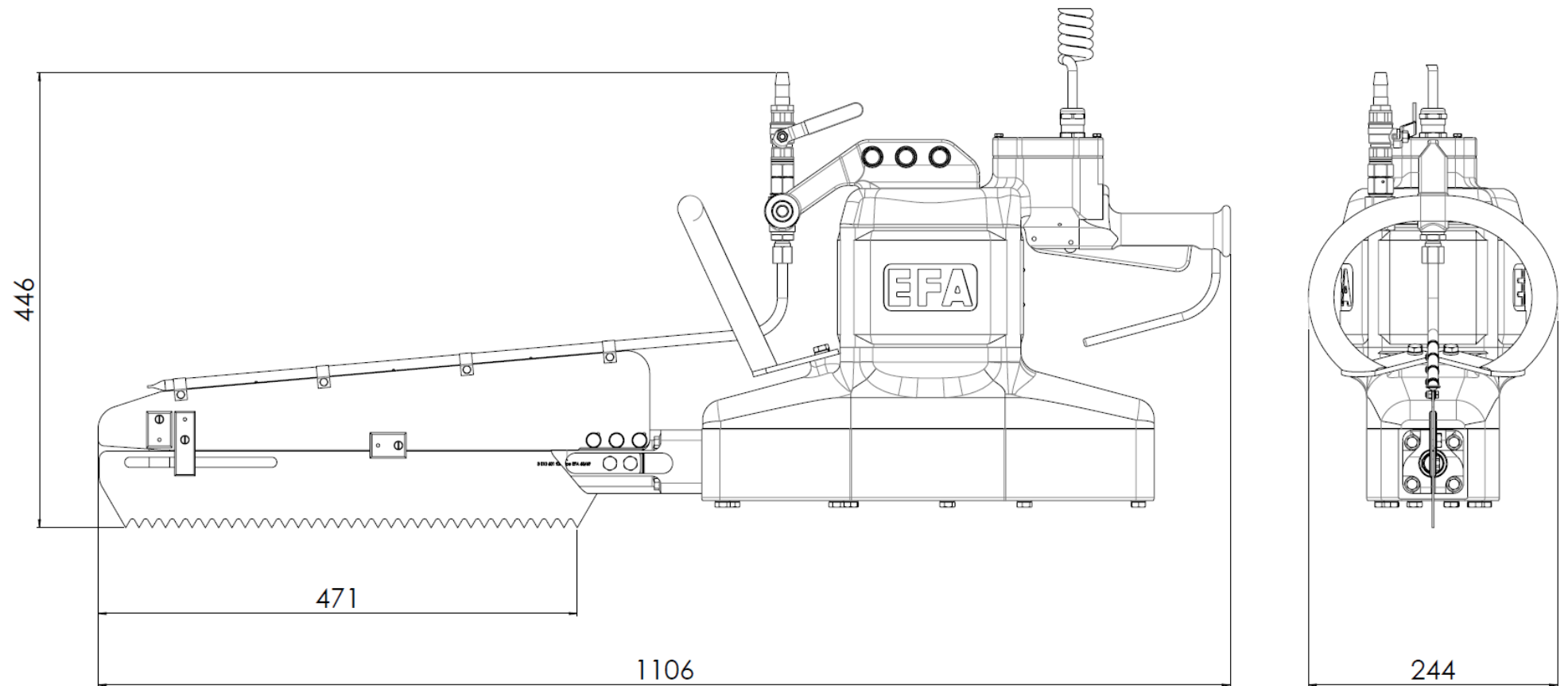
Dimensional drawing
